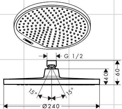
Crometta S 240 1jet 26723000
