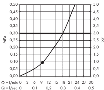
Crometta S 240 1jet 26723000
